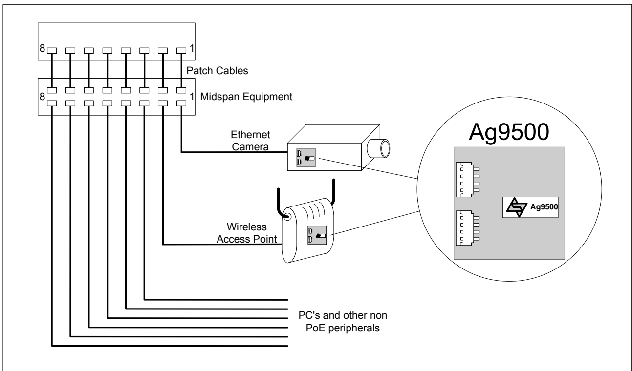
Figure 6: Typical Application
