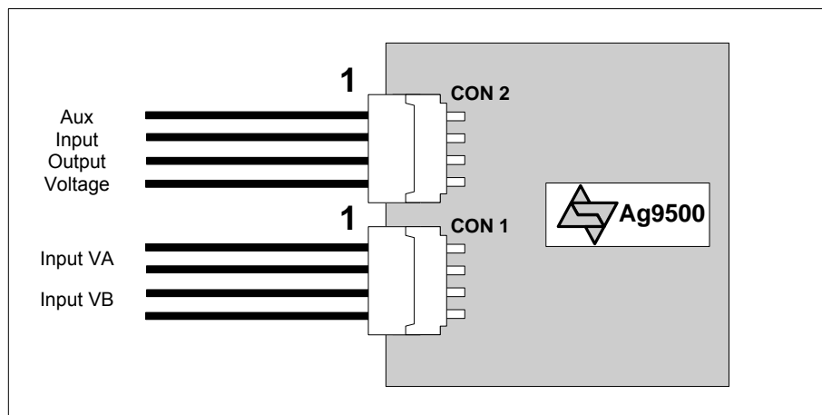
Figure 7: Typical Connection
