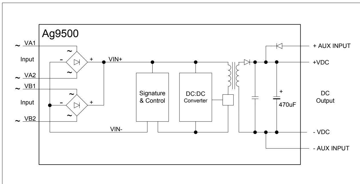
Figure 1: Block Diagram
